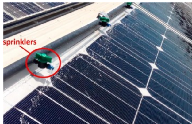
Figure 22. Visual of high- pressure sprinkler head for solar panel cooling system (Castanheira A., Fernandes J., Branco C., 2018)
