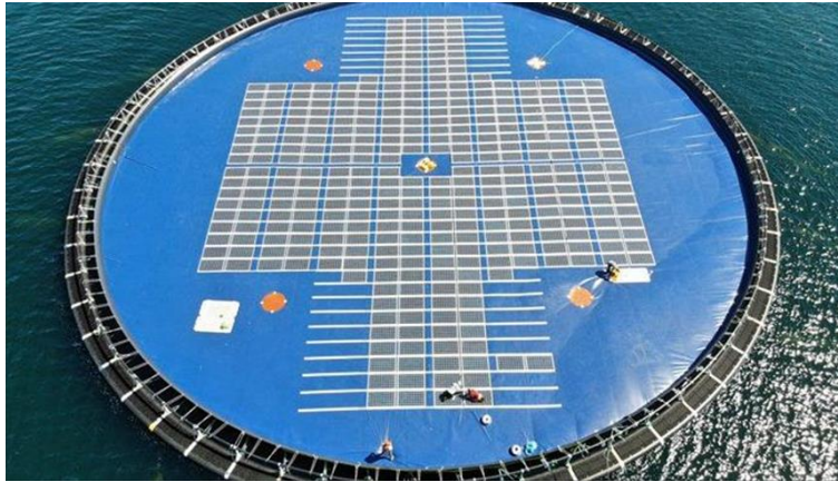
Figure 27. Swimming Solar Park by Statkraft, Albania
