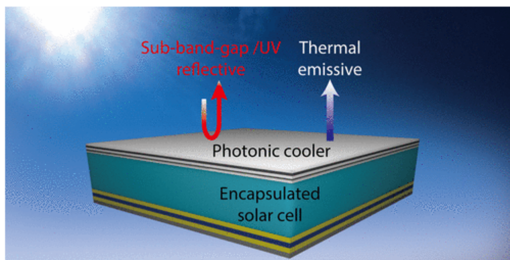
Figure 24. Diagram of Photonic Crystal Cooling Material (Li W., Shi Y., Chen K., Zhu L., Fan S., 2017)
