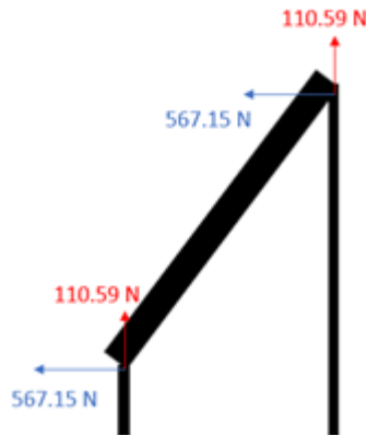
Figure 49. Forces on Each Leg from Wind and Weight of Panels and Mirrors
