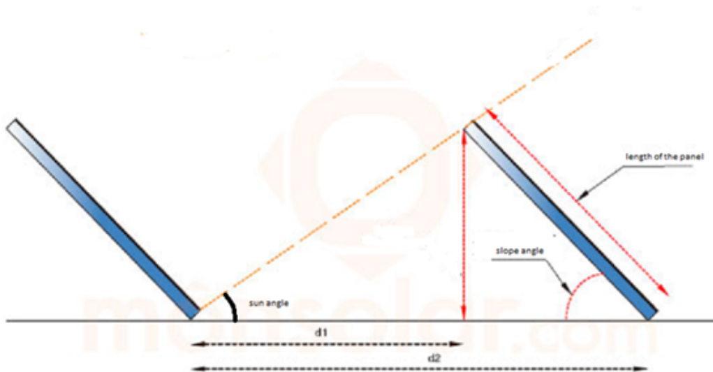
Figure 8. Diagram of position of panels
