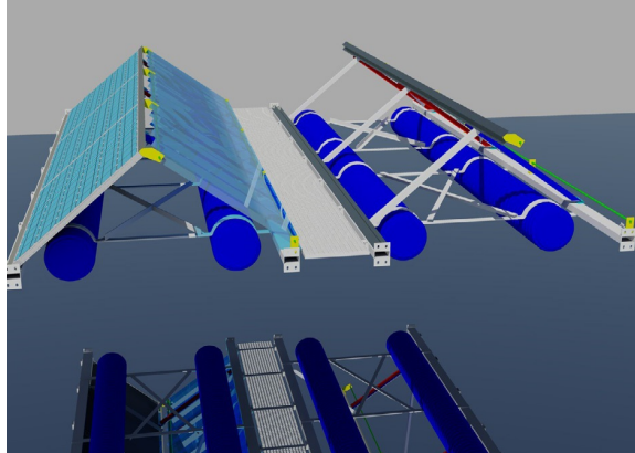
Figure 26. Submerged & floating photovoltaic systems
